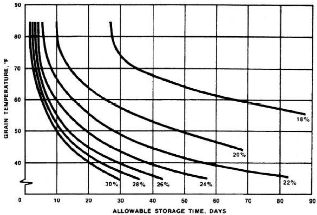
FIG. 1 — CORN STORAGE TIME AS A FUNCTION OF MOISTURE CONTENT AND TEMPERATURE (USDA)
